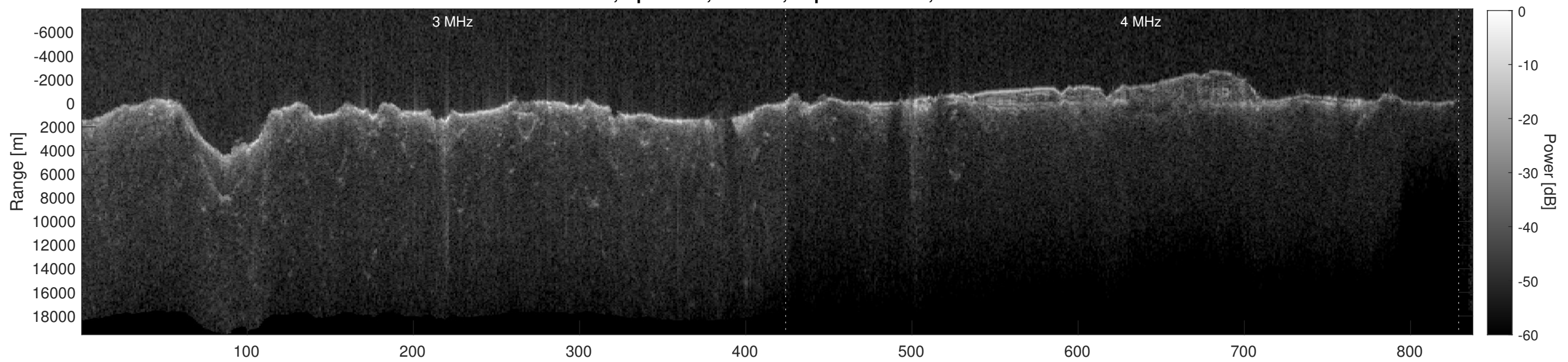
Orbit 6688, Depth-Corrected Cluttergram
