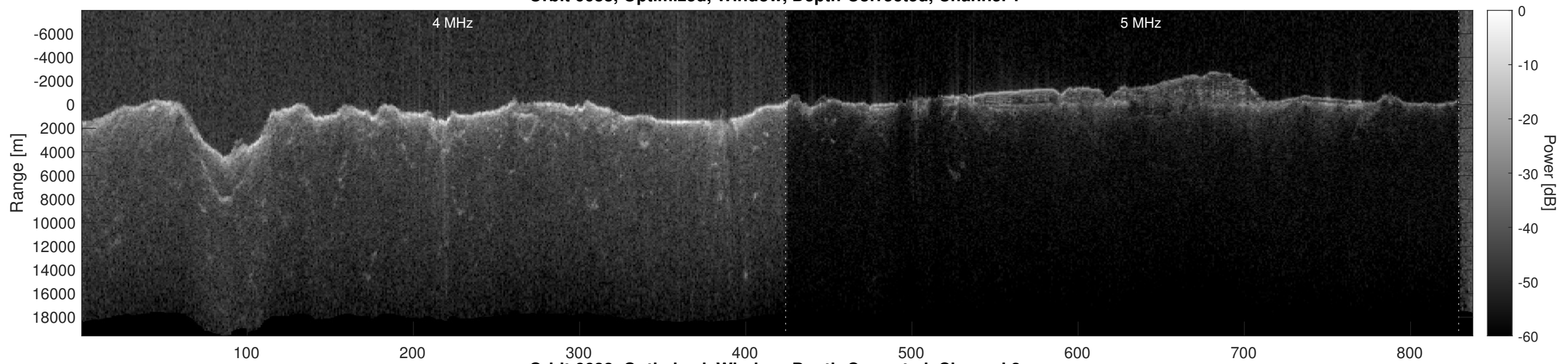
Orbit 6688, Optimized, Window, Depth-Corrected, Channel 2
