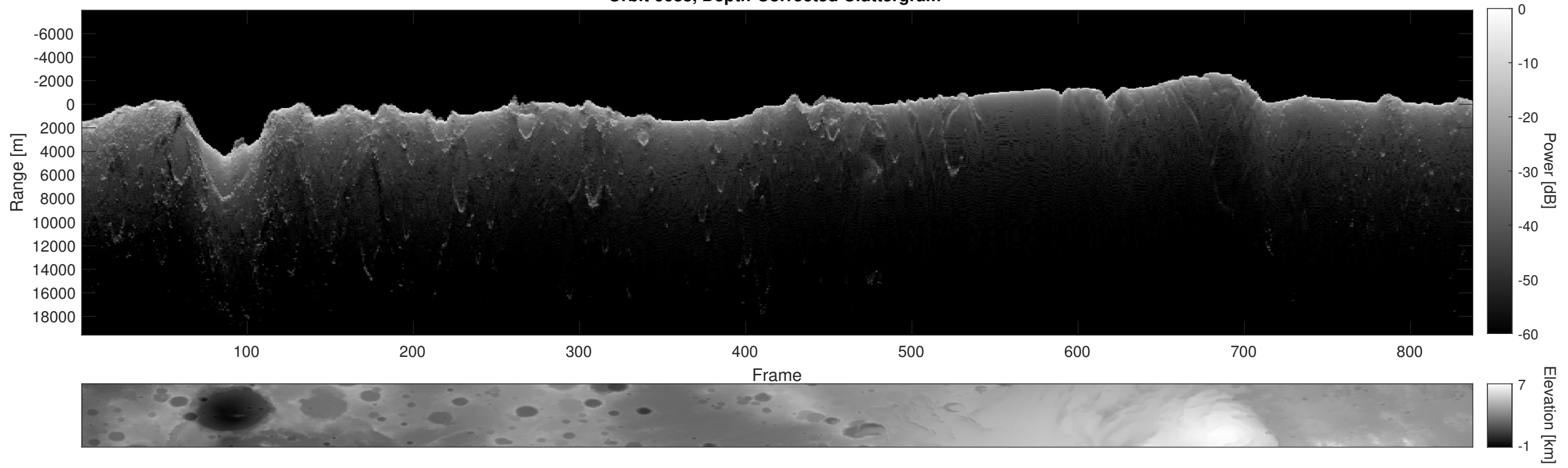
Orbit 6688, Depth-Corrected Cluttergram
