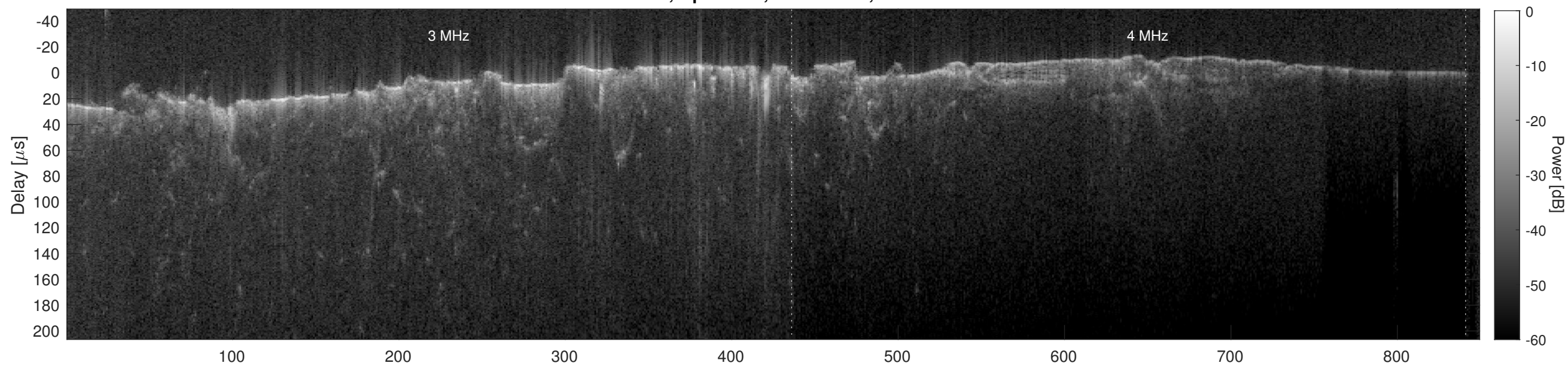
Orbit 6689, Cluttergram
