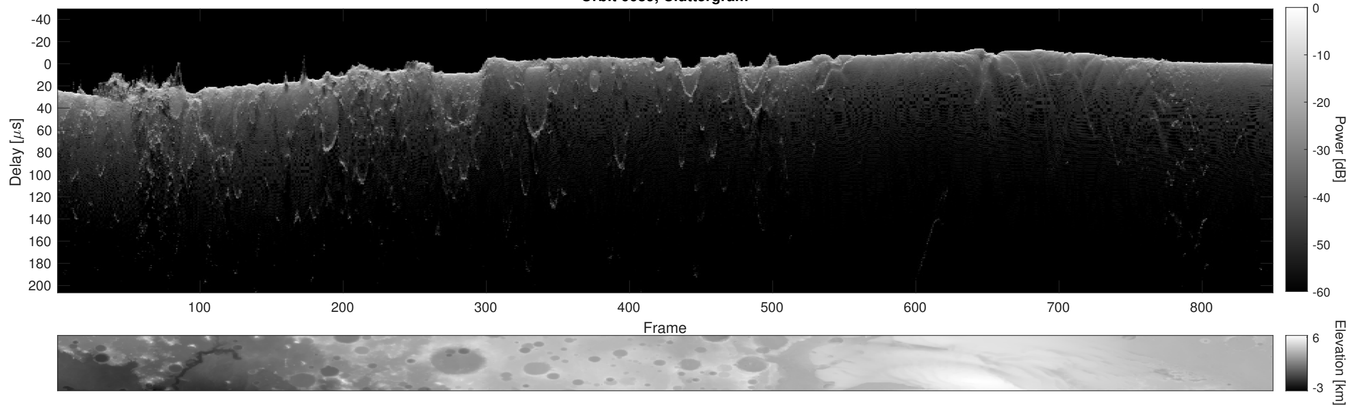
Orbit 6689, Cluttergram
