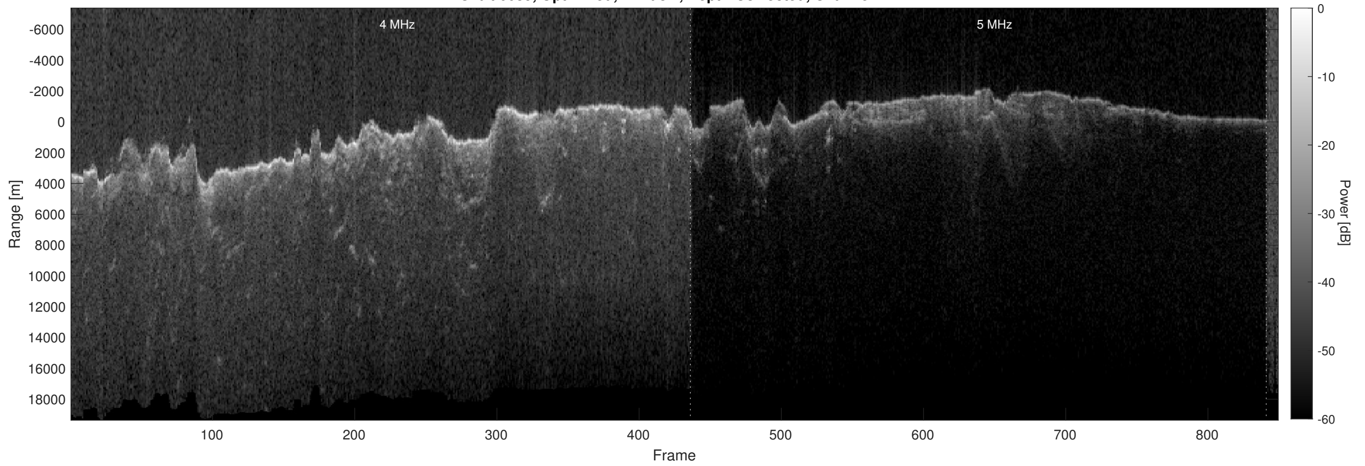
Orbit 6689, Optimized, Window, Depth-Corrected, Channel 2
