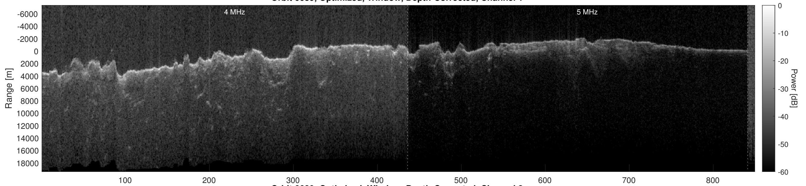
Orbit 6689, Optimized, Window, Depth-Corrected, Channel 2
