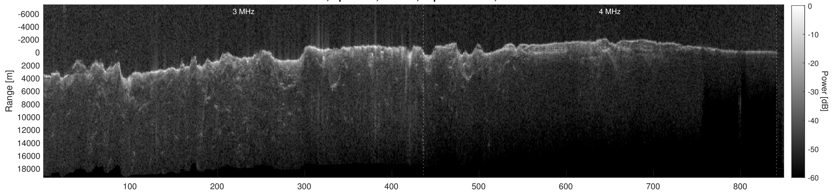
Orbit 6689, Depth-Corrected Cluttergram
