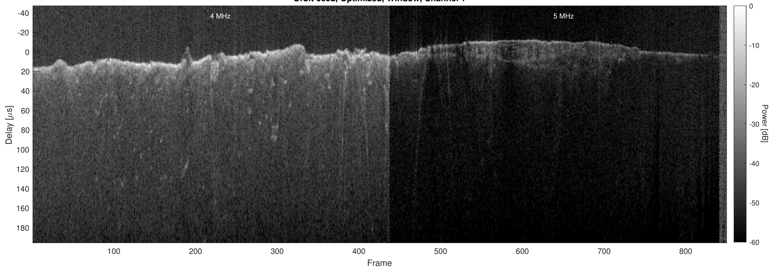
Orbit 6692, Optimized, Window, Channel 2
