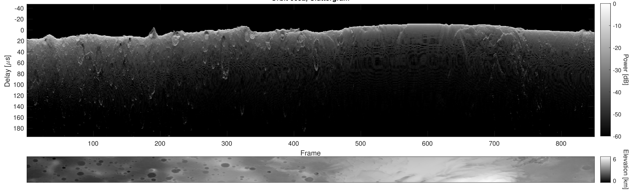
Orbit 6692, Cluttergram
