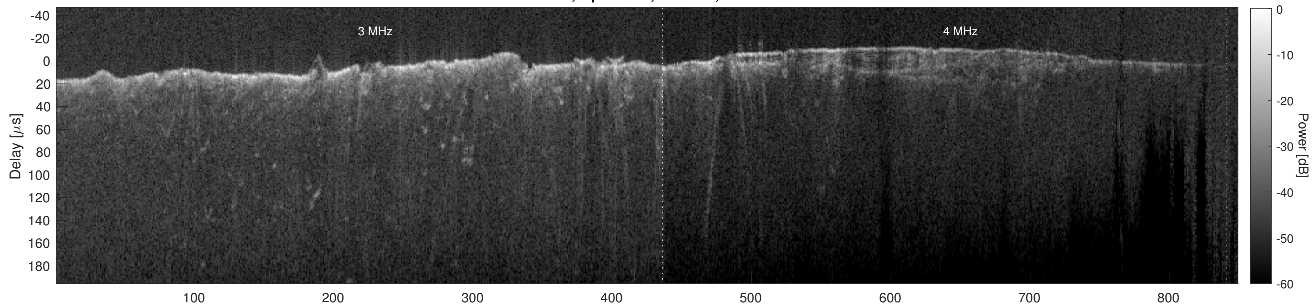
Orbit 6692, Cluttergram
