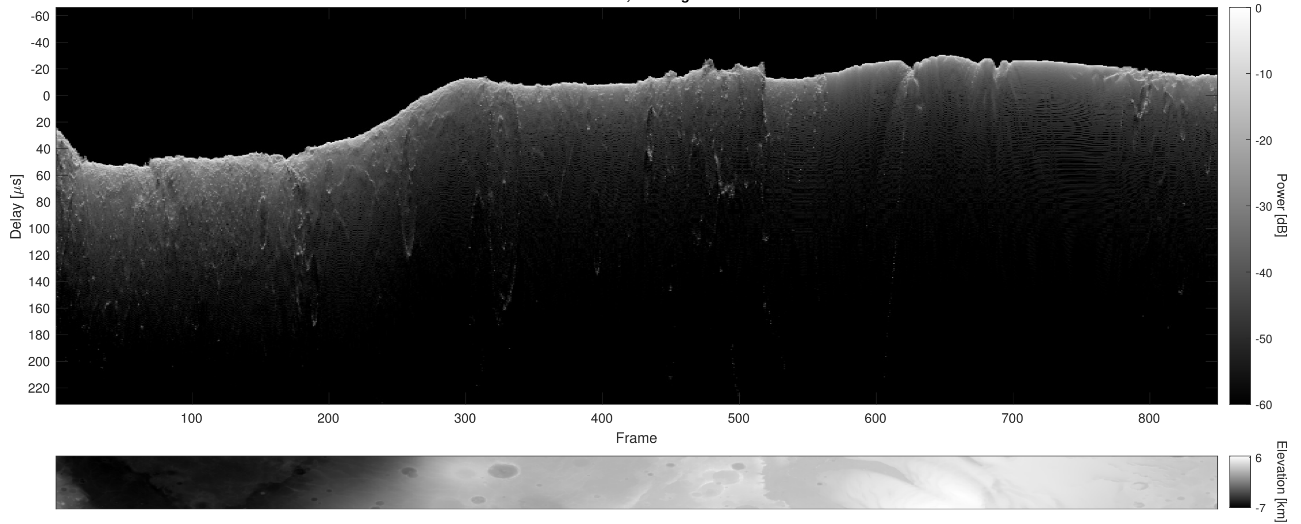
Orbit 6693, Cluttergram
