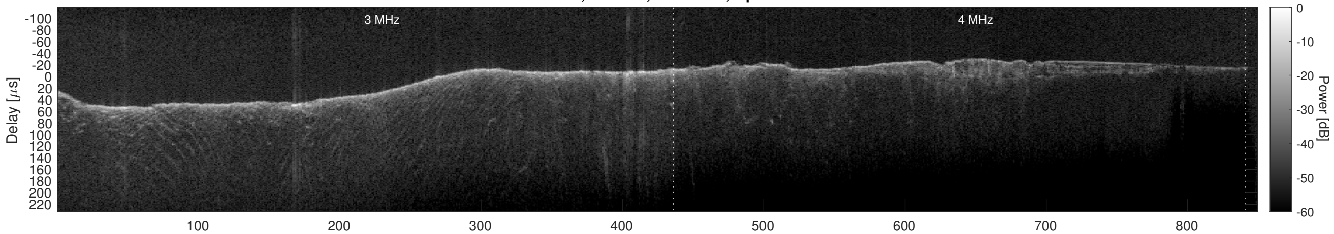
Orbit 6693, Cluttergram
