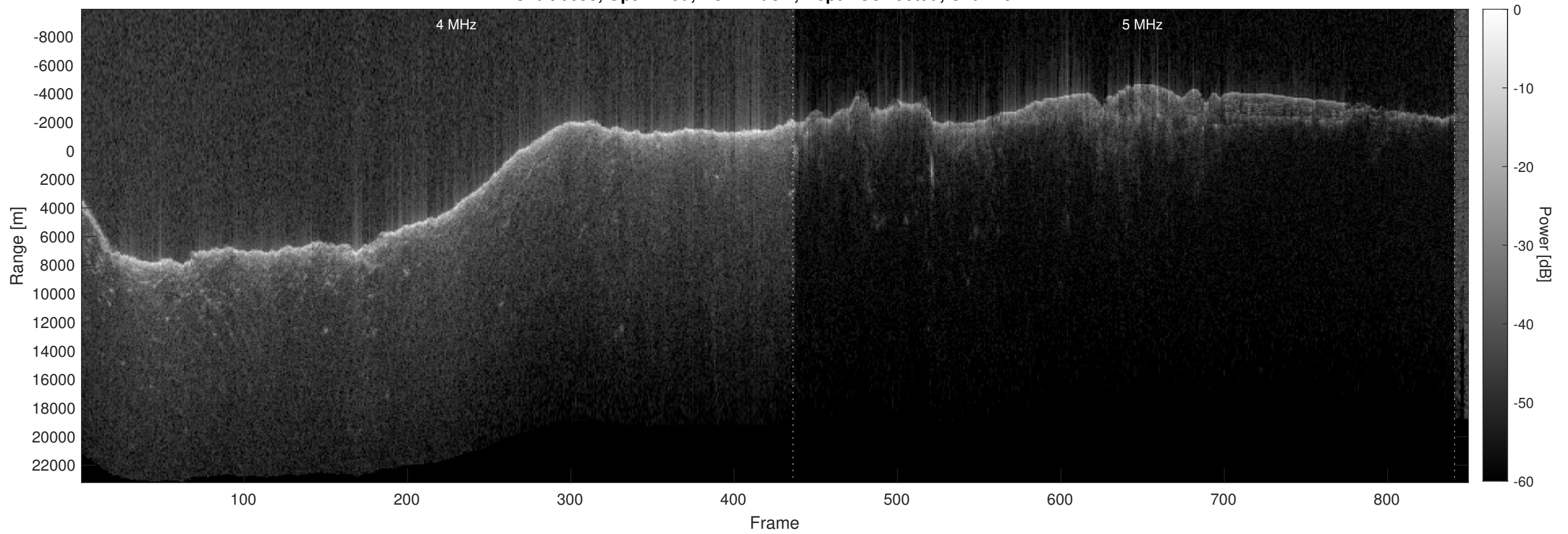
Orbit 6693, Optimized, No Window, Depth-Corrected, Channel 2
