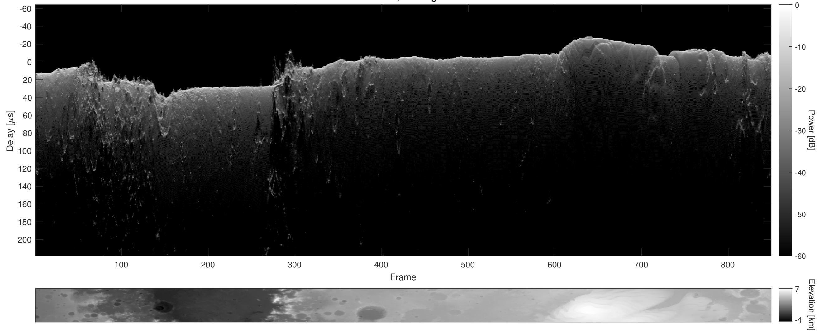
Orbit 6694, Cluttergram
