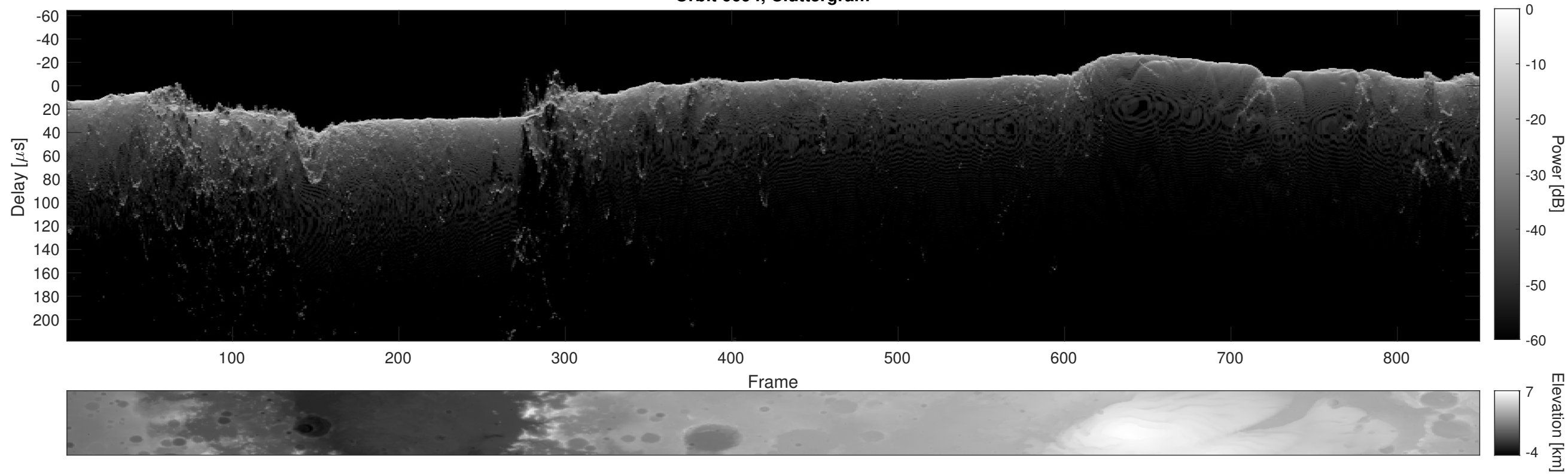
Orbit 6694, Cluttergram
