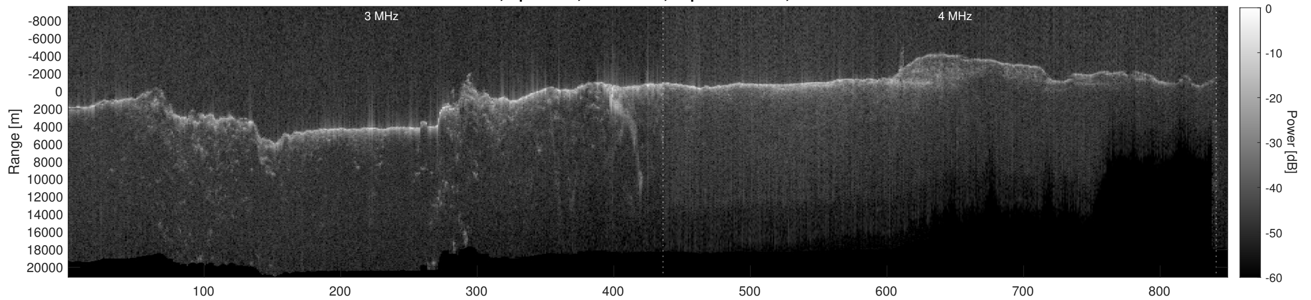
Orbit 6694, Depth-Corrected Cluttergram
