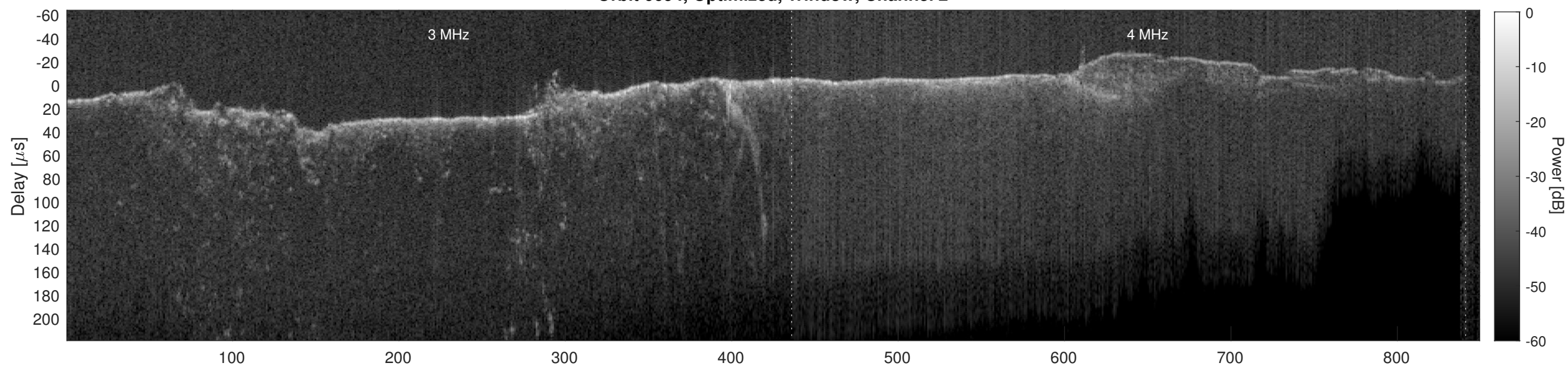
Orbit 6694, Cluttergram
