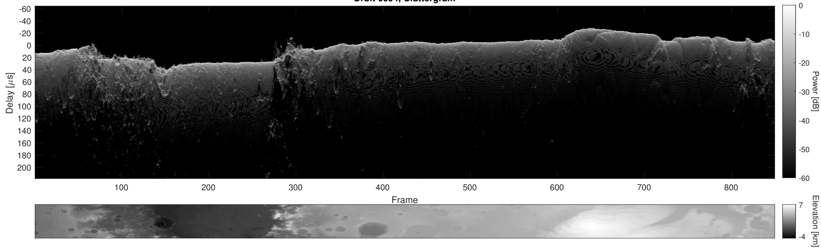
Orbit 6694, Cluttergram
