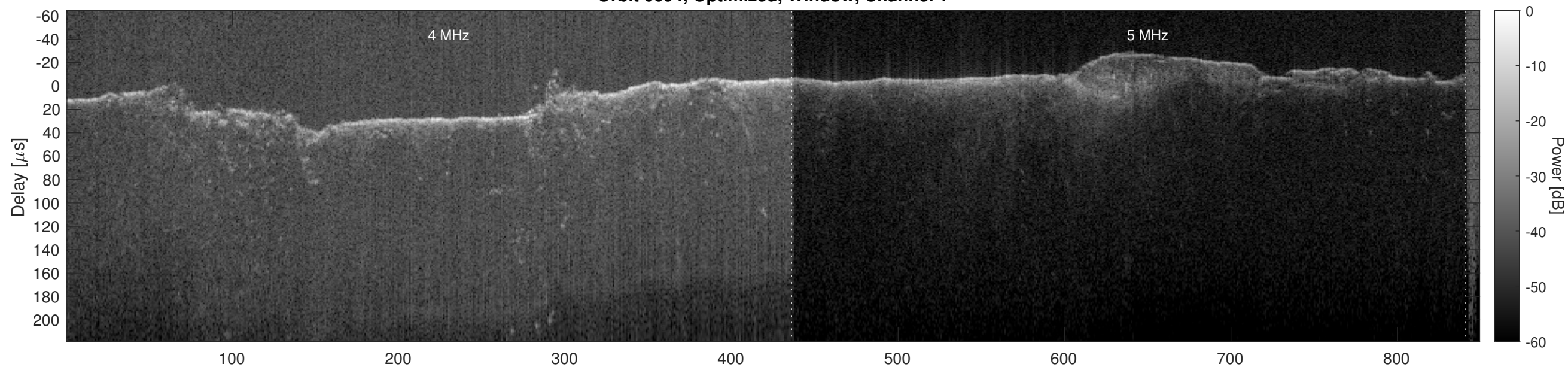
Orbit 6694, Optimized, Window, Channel 2
