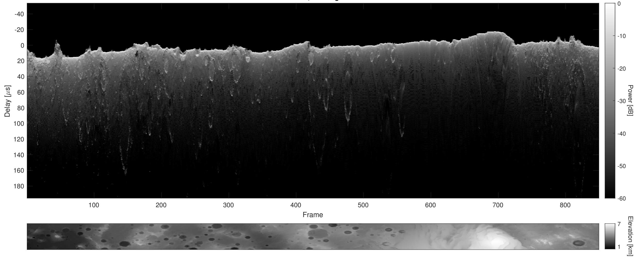
Orbit 6695, Cluttergram
