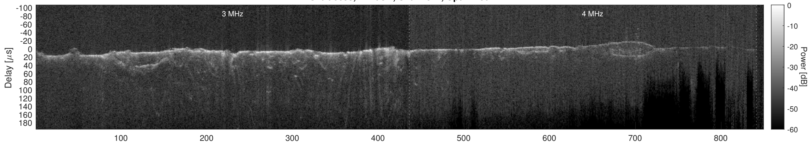
Orbit 6695, Cluttergram
