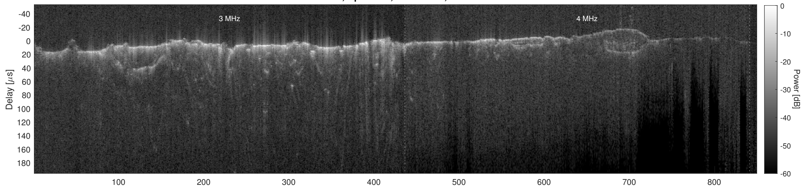
Orbit 6695, Cluttergram
