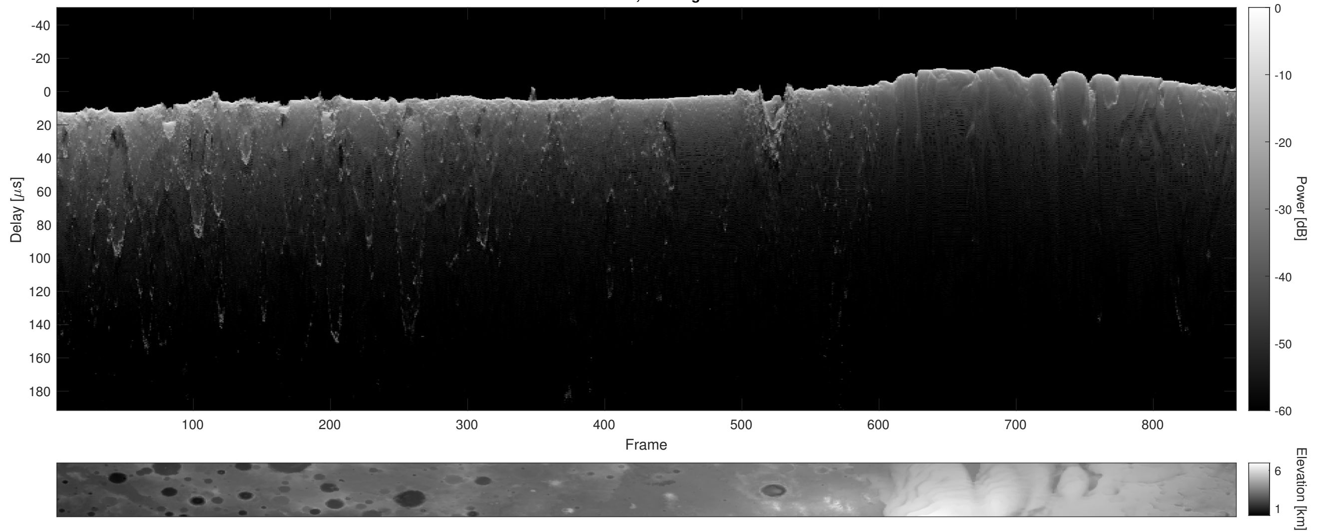
Orbit 6697, Cluttergram
