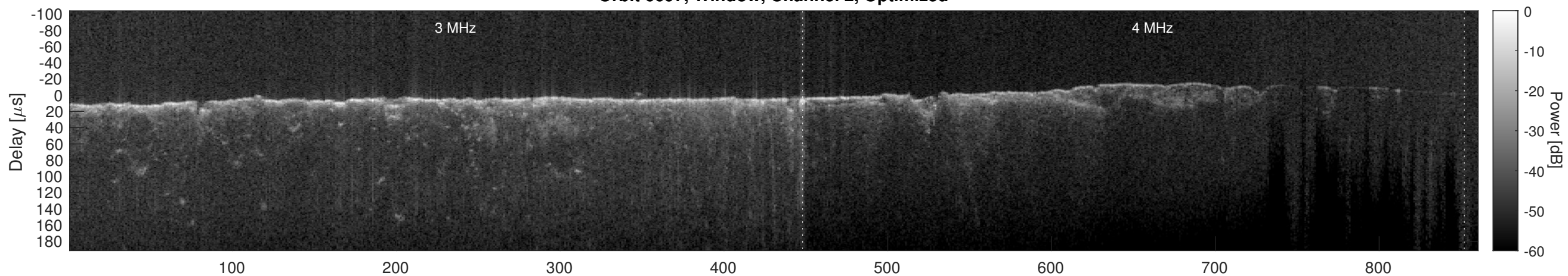
Orbit 6697, Cluttergram
