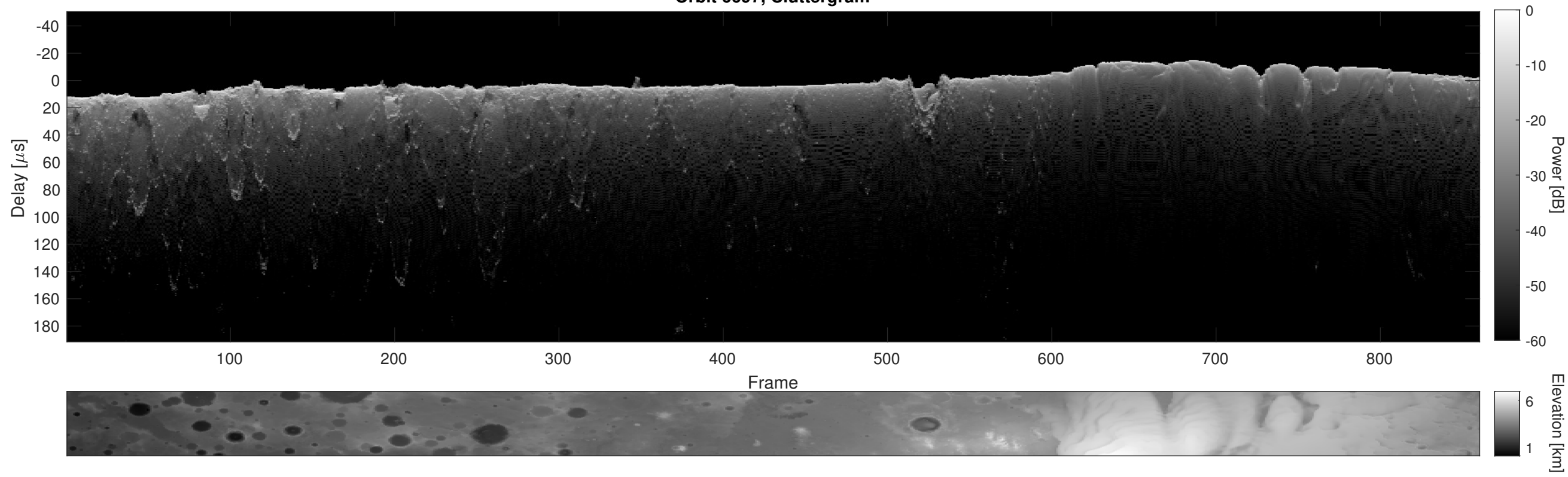
Orbit 6697, Cluttergram
