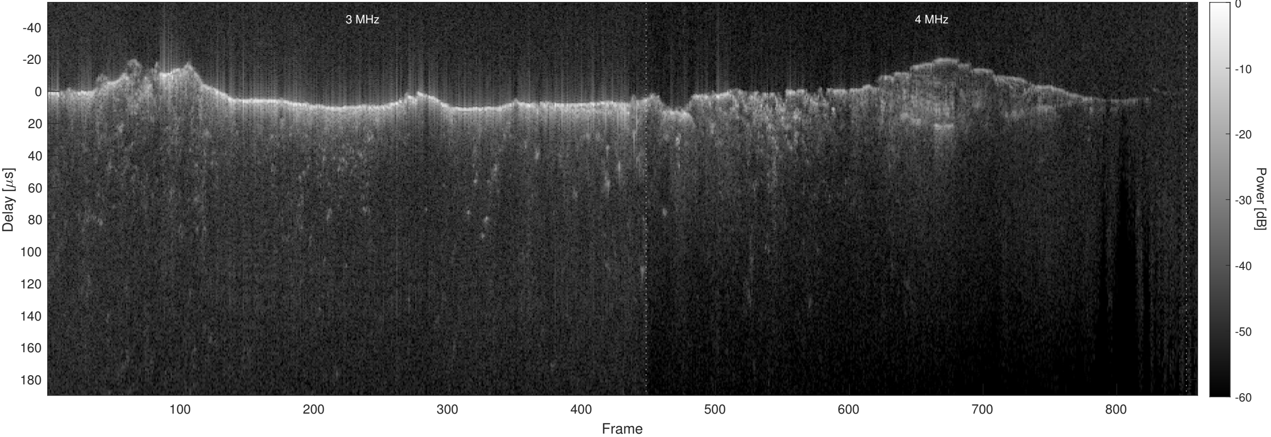
Orbit 6698, Optimized, No Window, Channel 2
