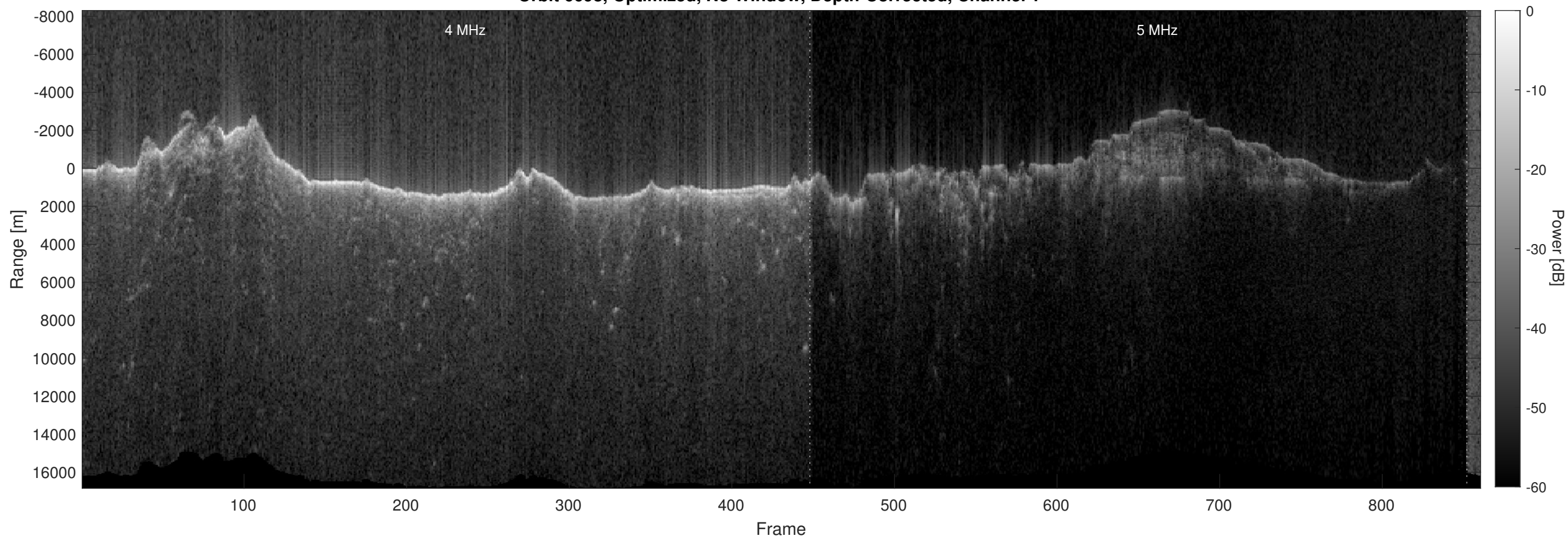
Orbit 6698, Optimized, No Window, Depth-Corrected, Channel 2
