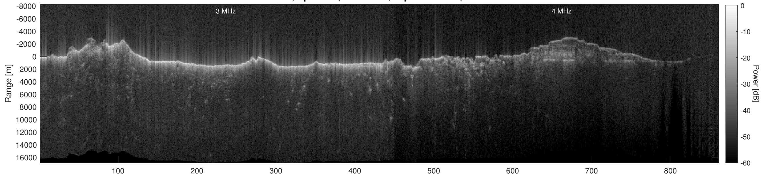
Orbit 6698, Depth-Corrected Cluttergram
