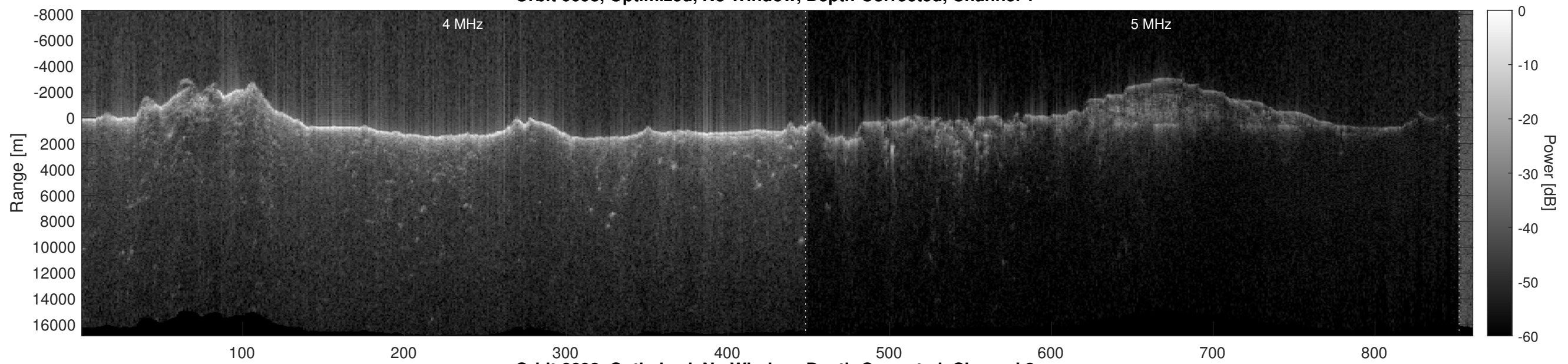
Orbit 6698, Optimized, No Window, Depth-Corrected, Channel 2
