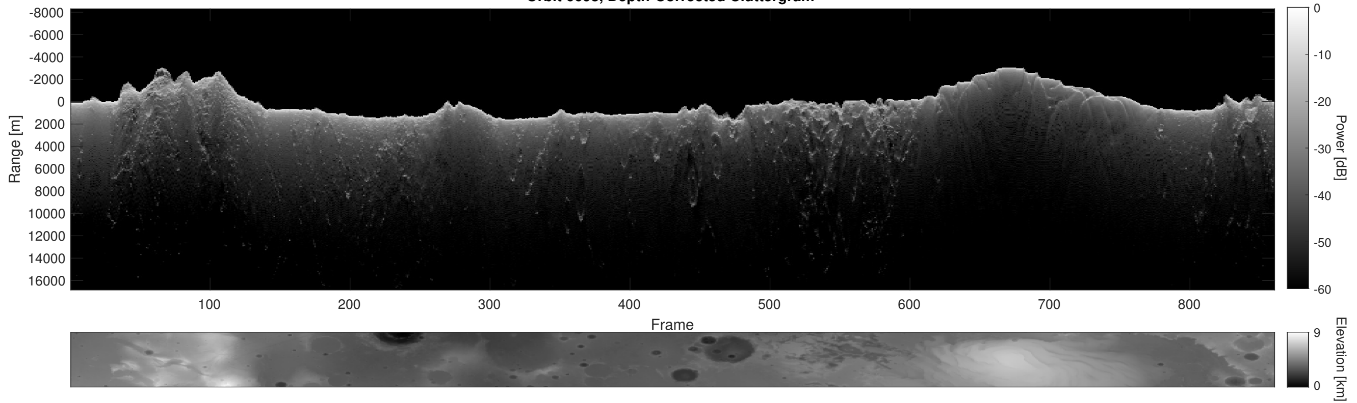
Orbit 6698, Depth-Corrected Cluttergram
