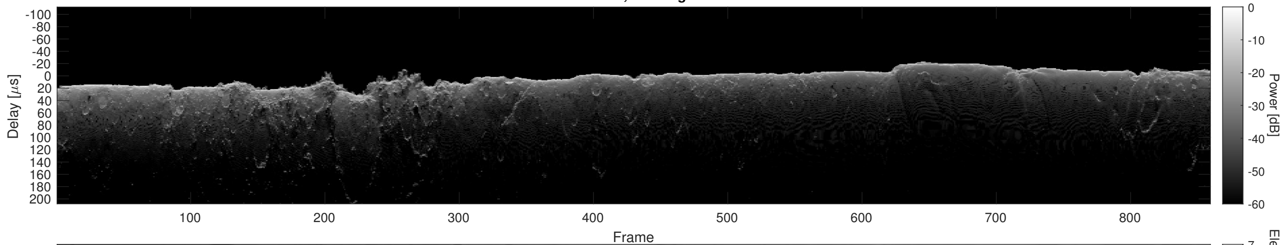
Orbit 6701, Cluttergram
