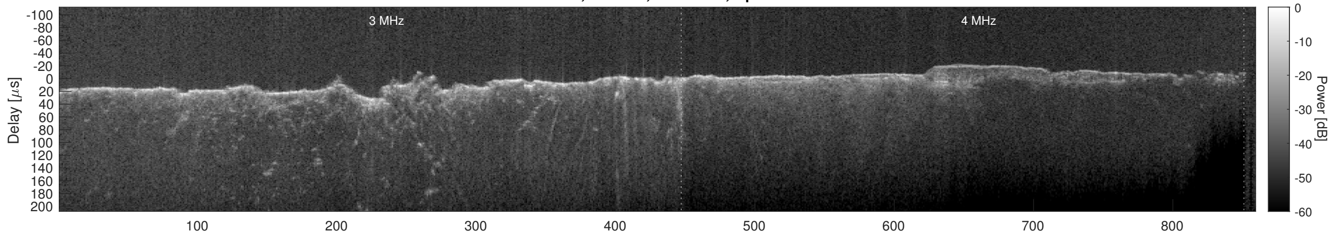
Orbit 6701, Cluttergram
