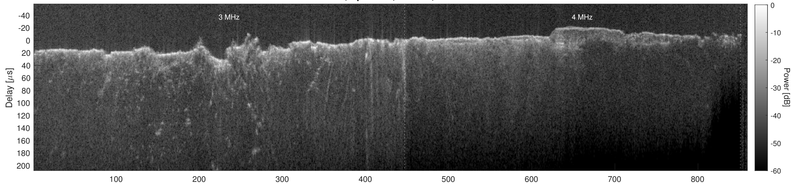
Orbit 6701, Cluttergram
