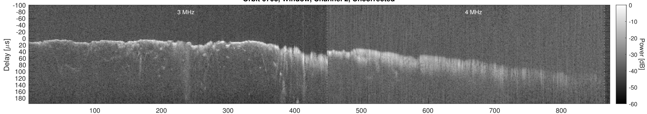
Orbit 6703, Window, Channel 2, Chapman
