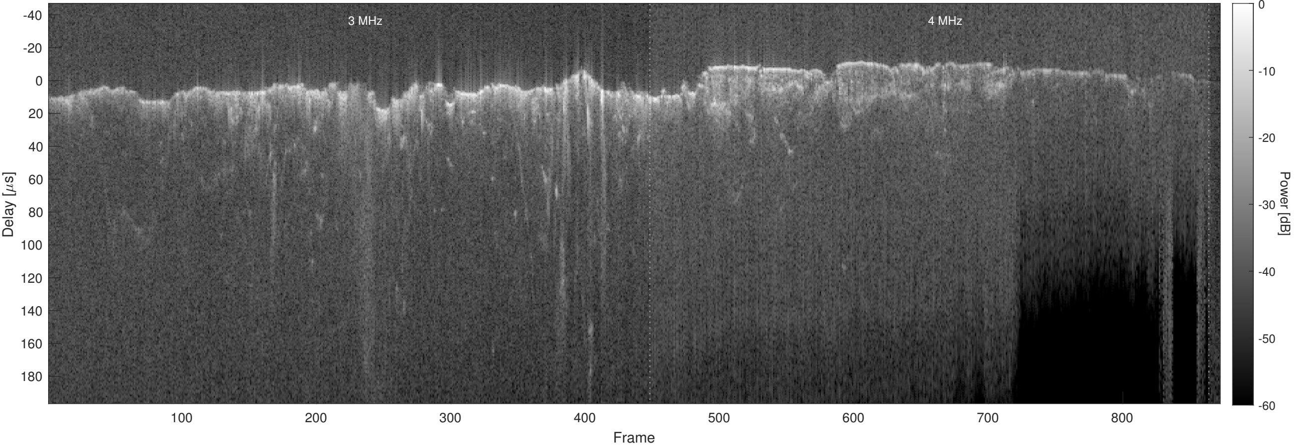
Orbit 6703, Optimized, No Window, Channel 2
