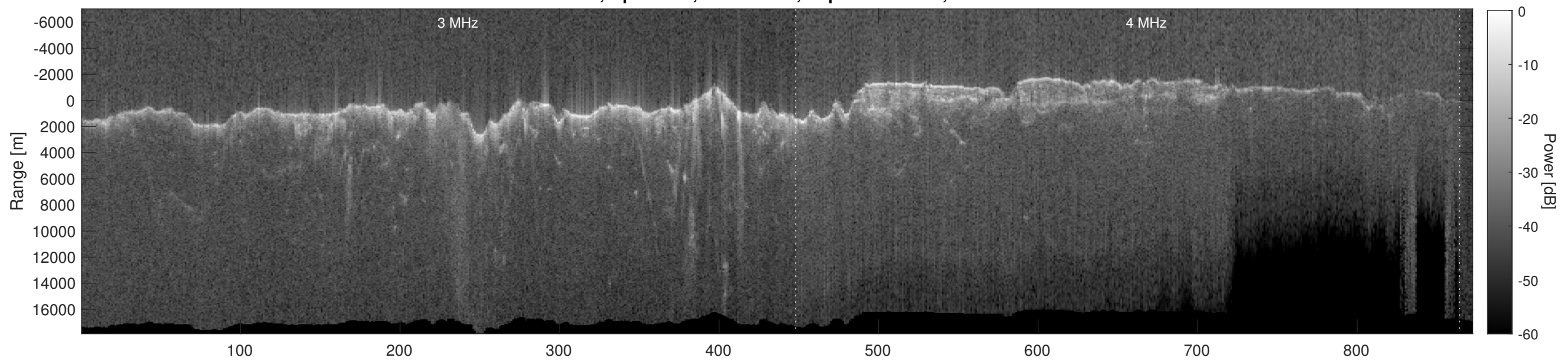
Orbit 6703, Depth-Corrected Cluttergram
