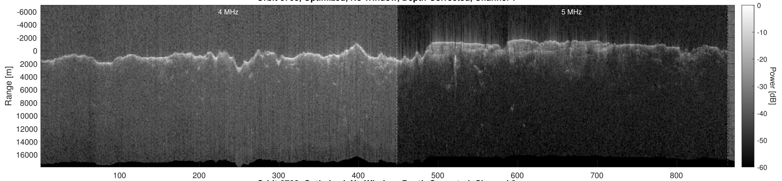
Orbit 6703, Optimized, No Window, Depth-Corrected, Channel 2
