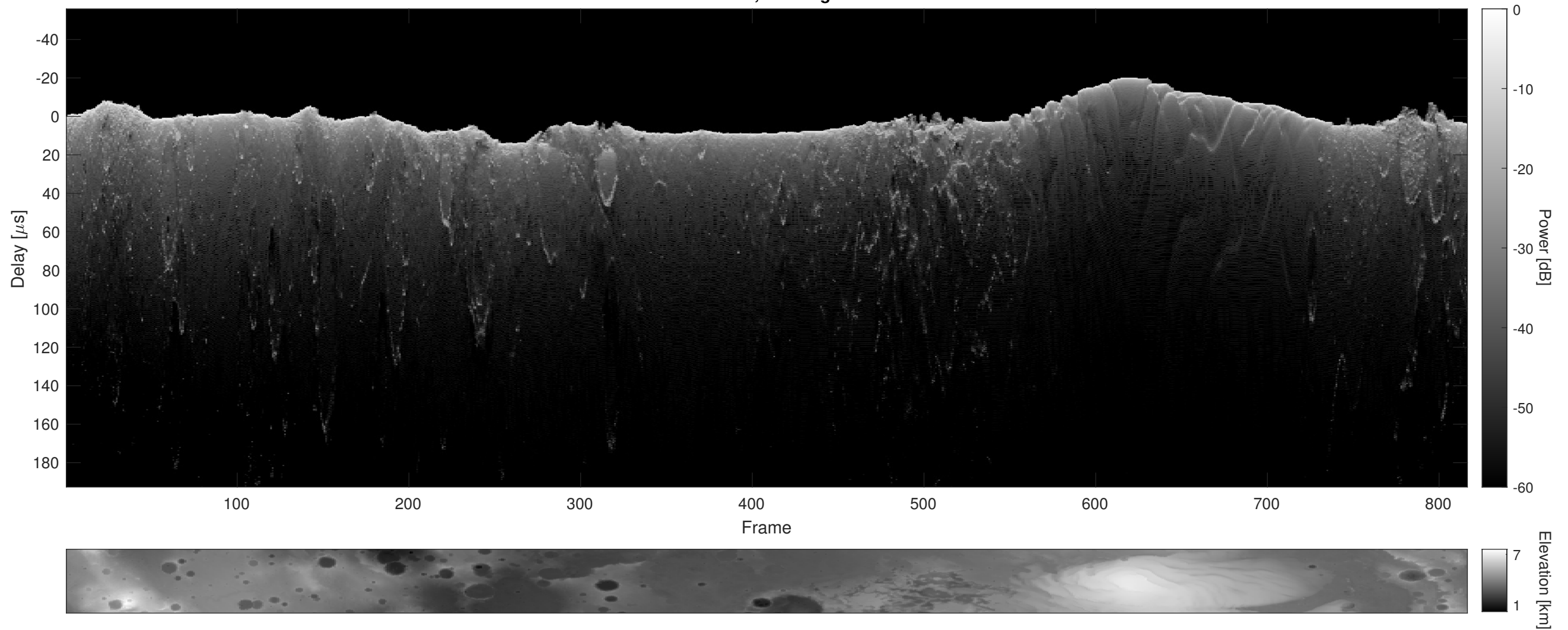
Orbit 6705, Cluttergram
