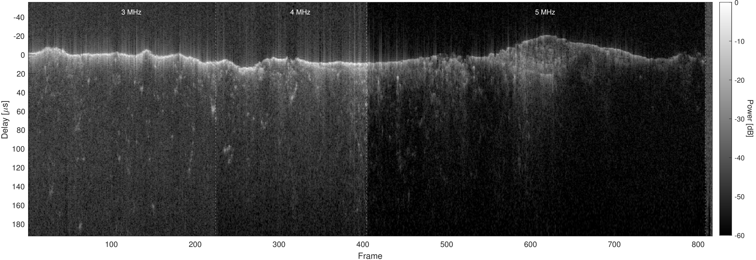
Orbit 6705, Optimized, No Window, Channel 2
