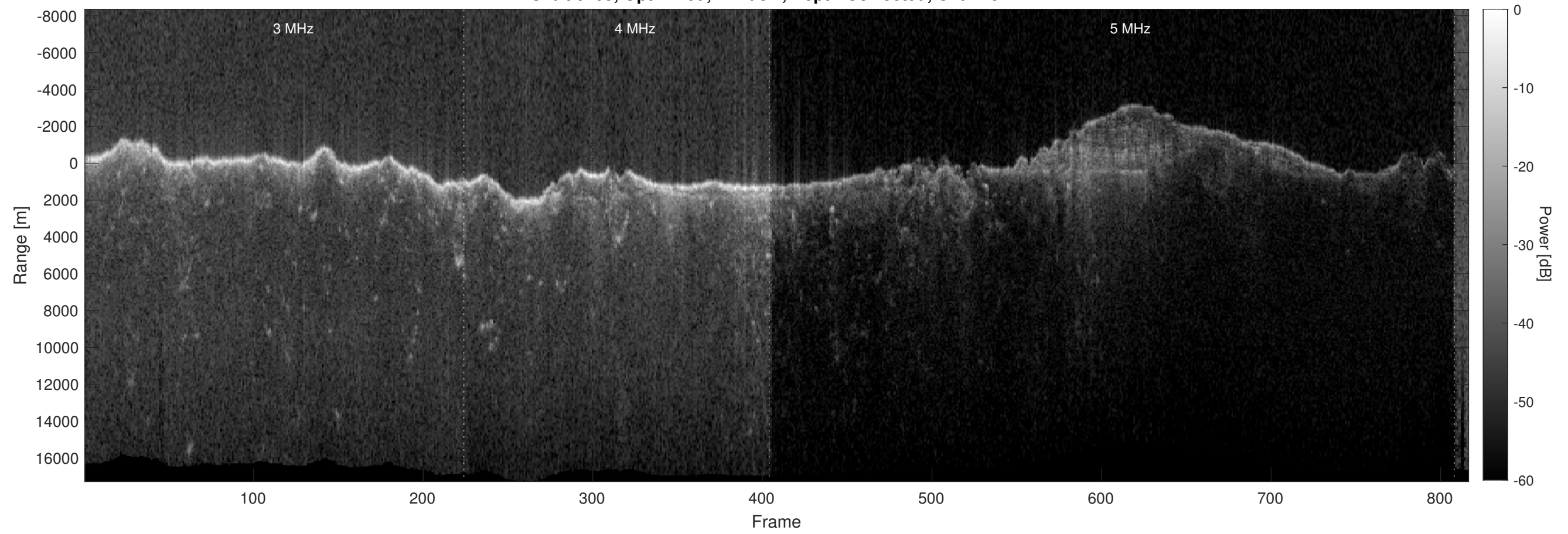
Orbit 6705, Optimized, Window, Depth-Corrected, Channel 2
