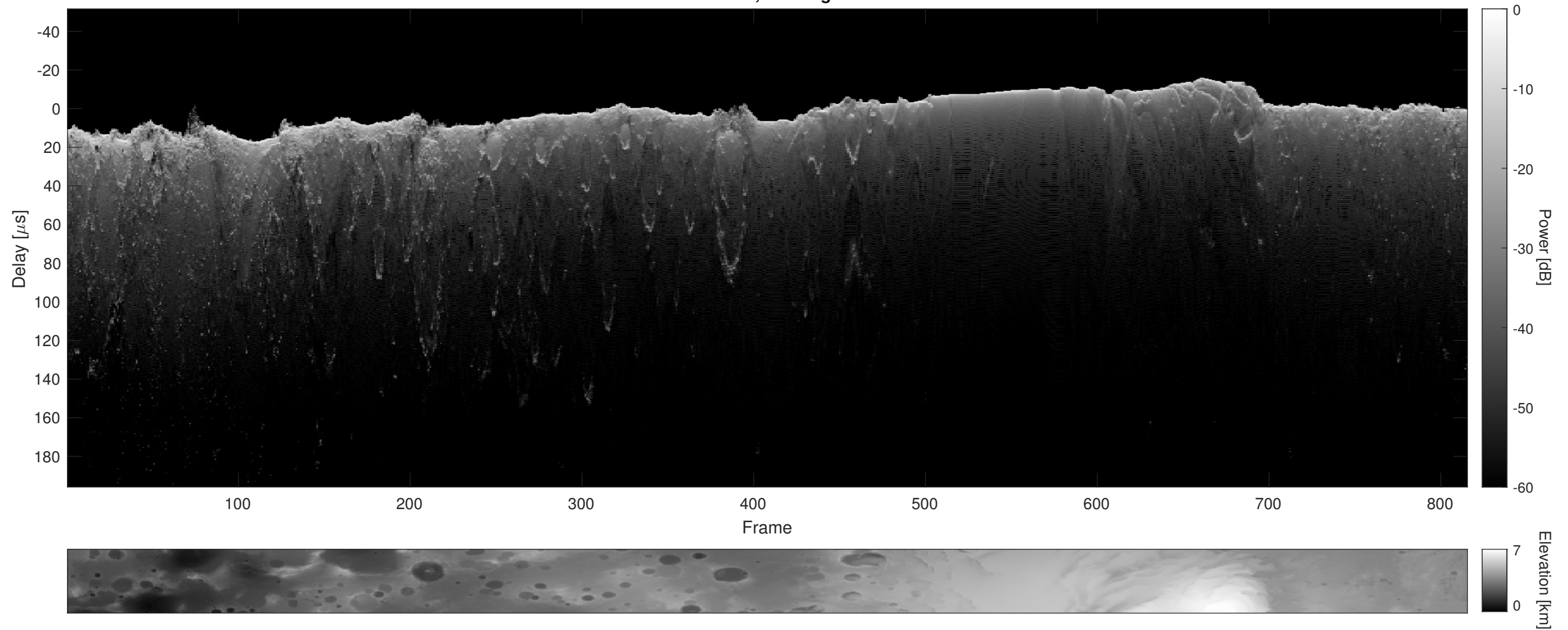
Orbit 6706, Cluttergram
