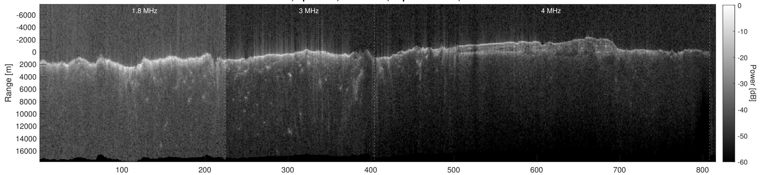
Orbit 6706, Depth-Corrected Cluttergram
