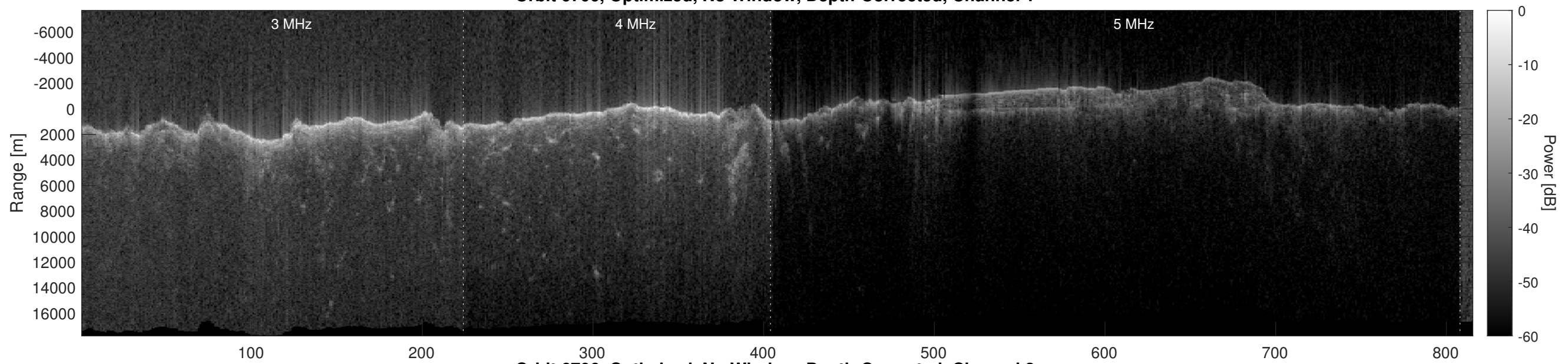
Orbit 6706, Optimized, No Window, Depth-Corrected, Channel 2
