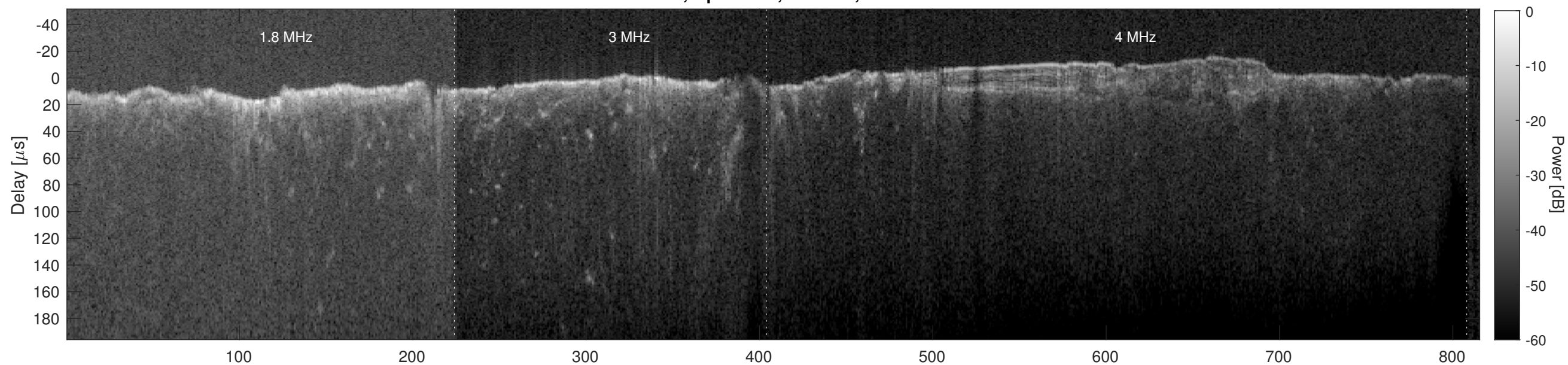
Orbit 6706, Cluttergram
