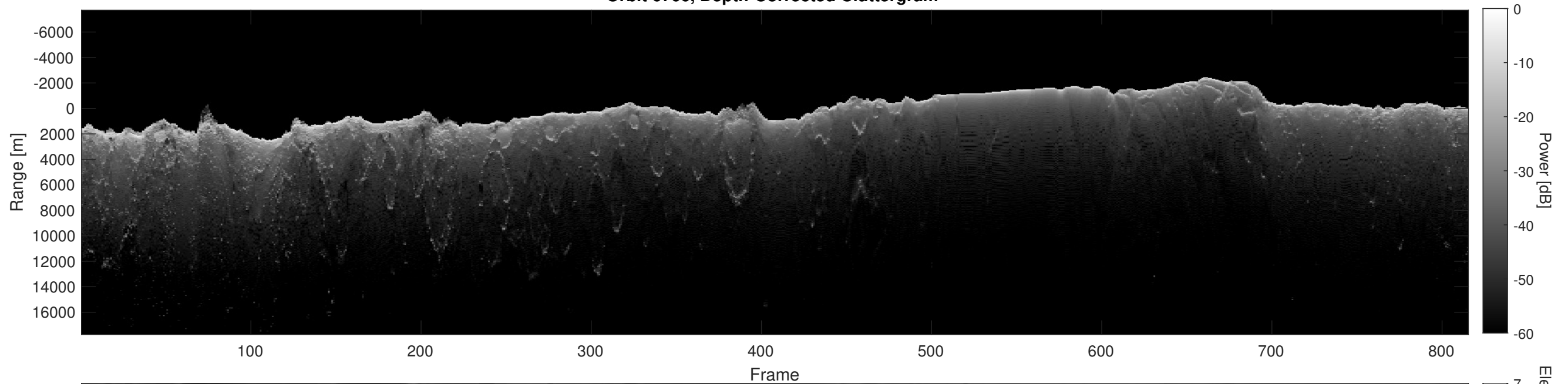
Orbit 6706, Depth-Corrected Cluttergram
