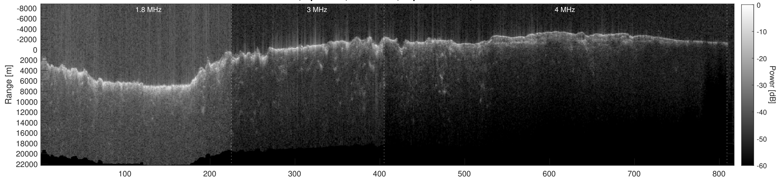
Orbit 6707, Depth-Corrected Cluttergram
