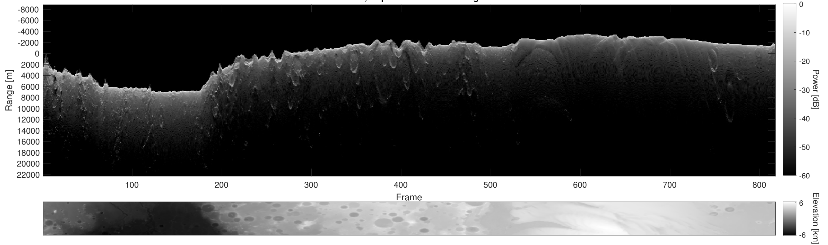
Orbit 6707, Depth-Corrected Cluttergram
