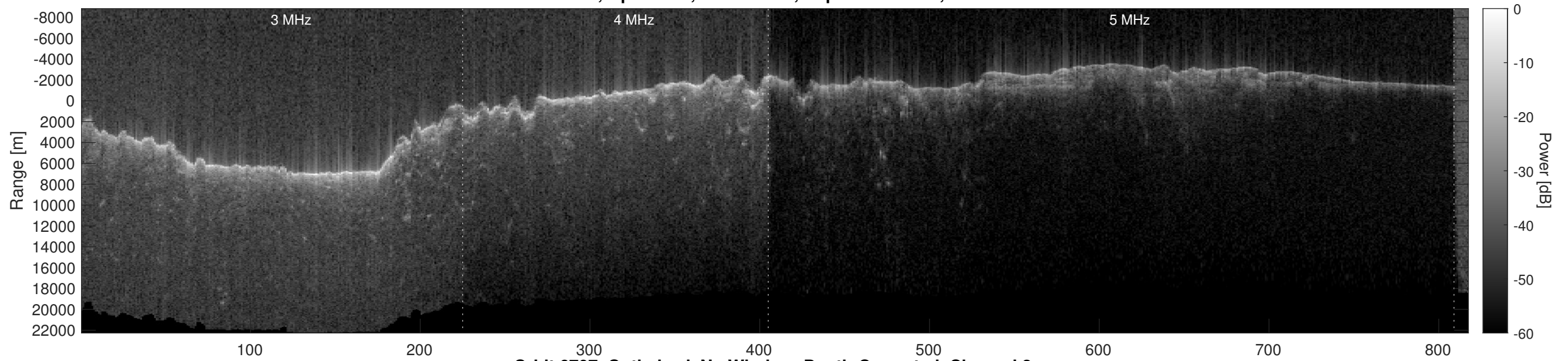
Orbit 6707, Optimized, No Window, Depth-Corrected, Channel 2
