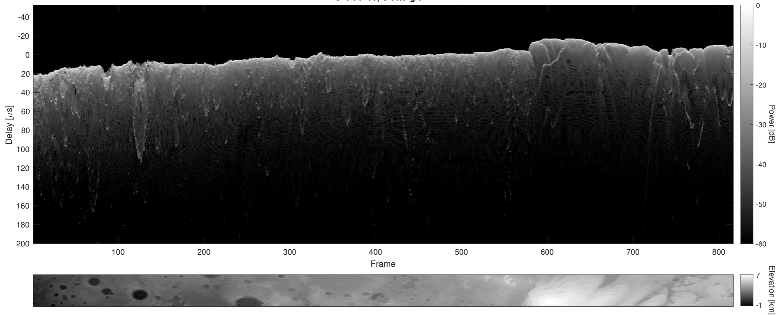
Orbit 6708, Cluttergram
