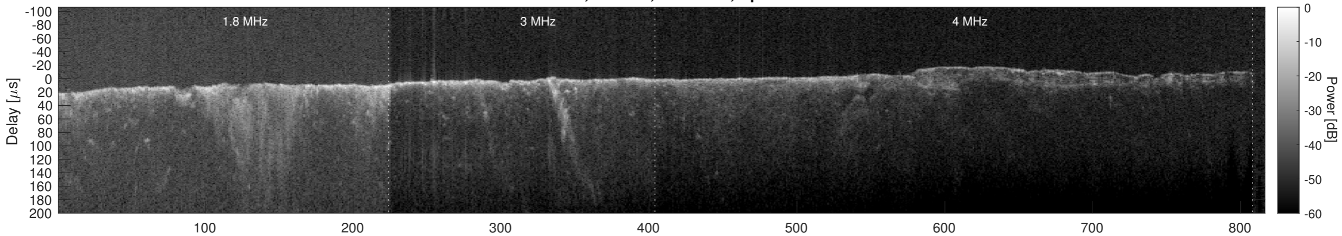
Orbit 6708, Cluttergram
