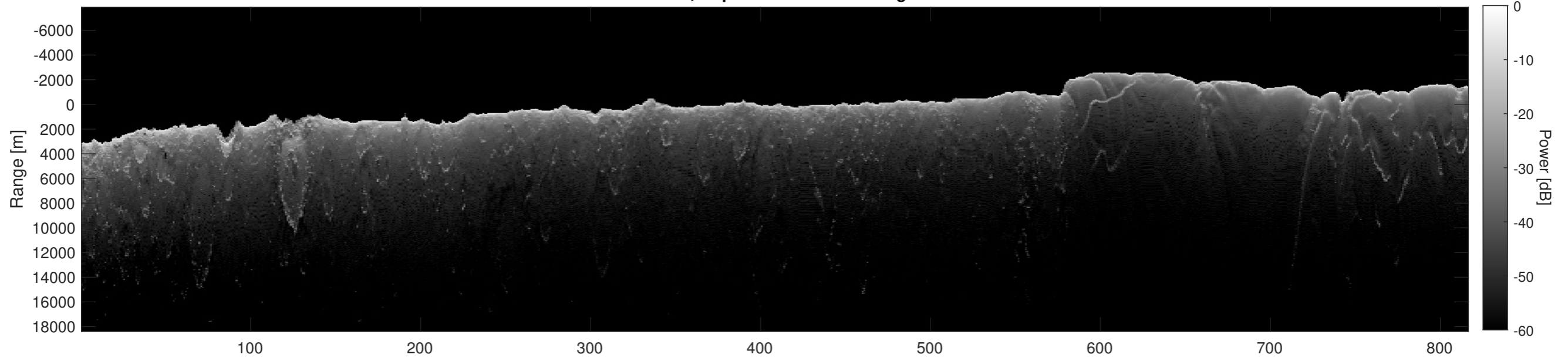
Orbit 6708, Depth-Corrected Cluttergram
