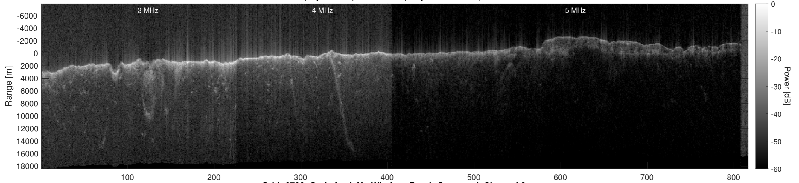
Orbit 6708, Optimized, No Window, Depth-Corrected, Channel 2
