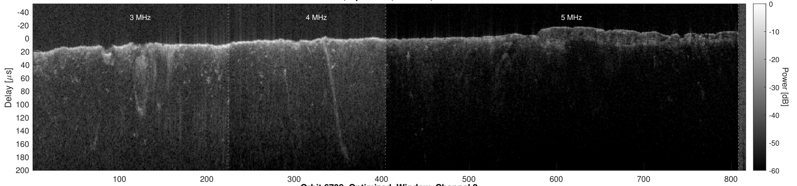
Orbit 6708, Optimized, Window, Channel 2
