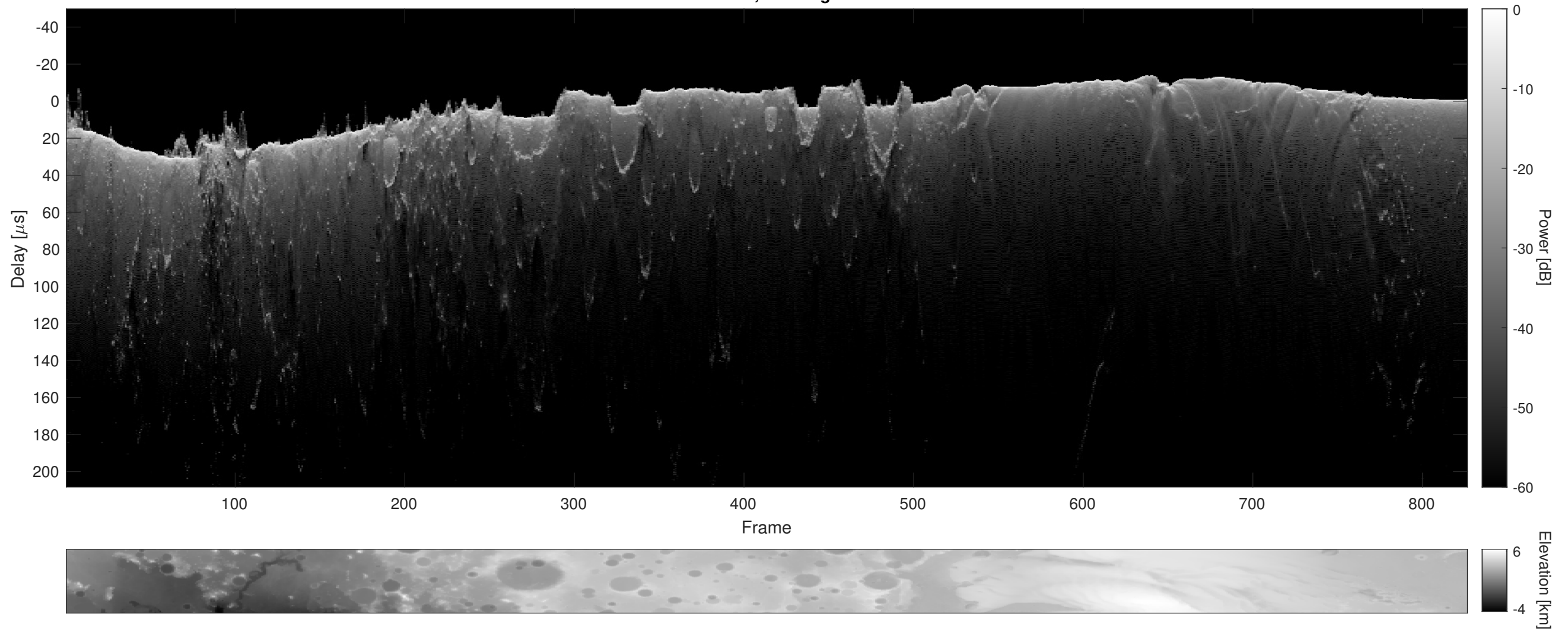
Orbit 6714, Cluttergram
