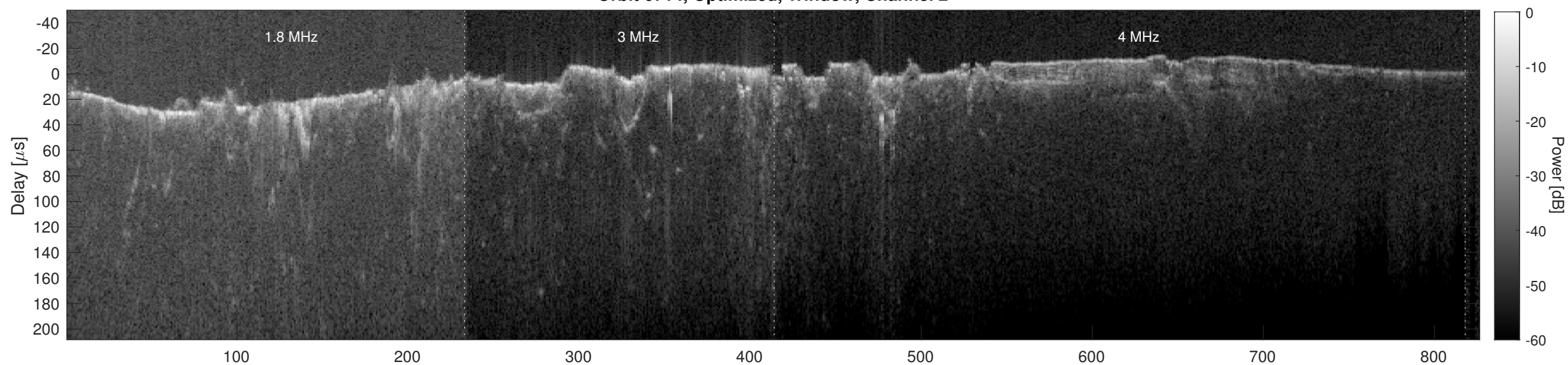
Orbit 6714, Cluttergram
