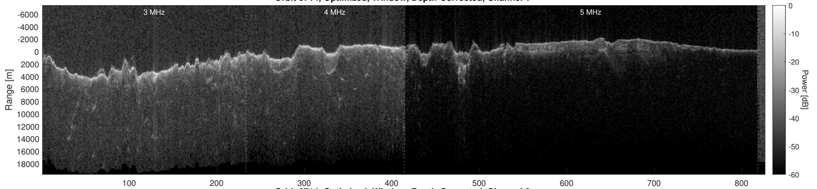
Orbit 6714, Optimized, Window, Depth-Corrected, Channel 2
