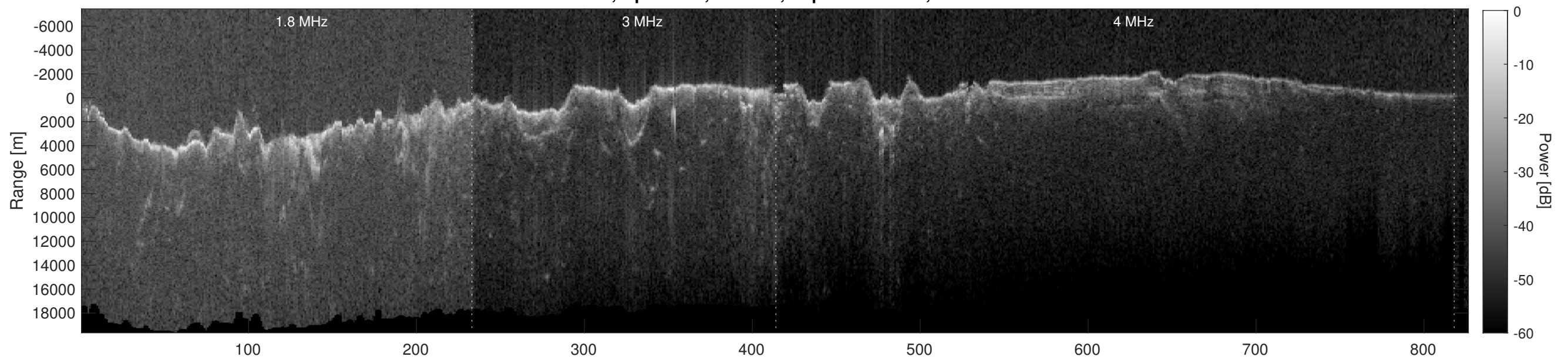
Orbit 6714, Depth-Corrected Cluttergram
