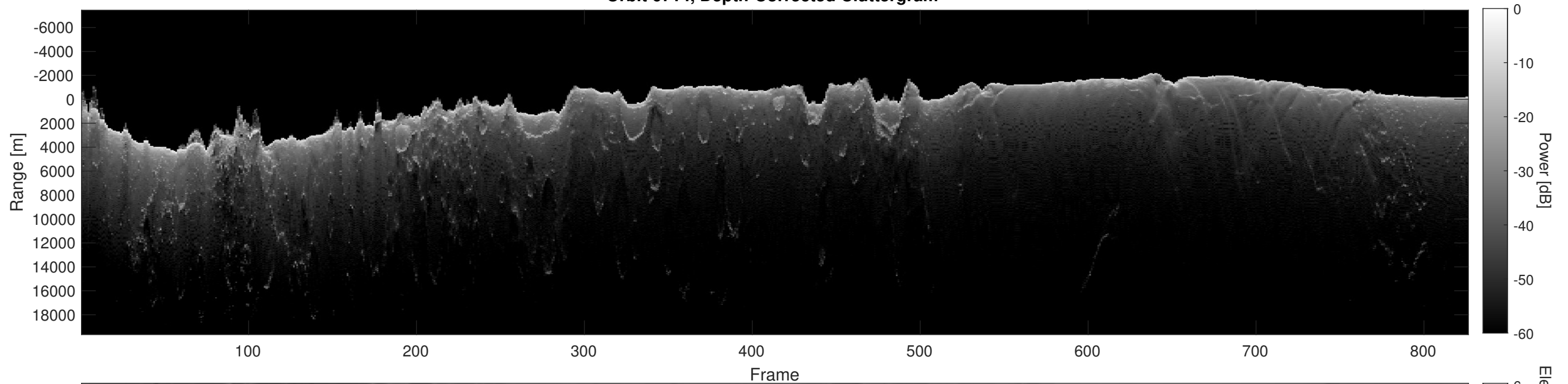
Orbit 6714, Depth-Corrected Cluttergram
