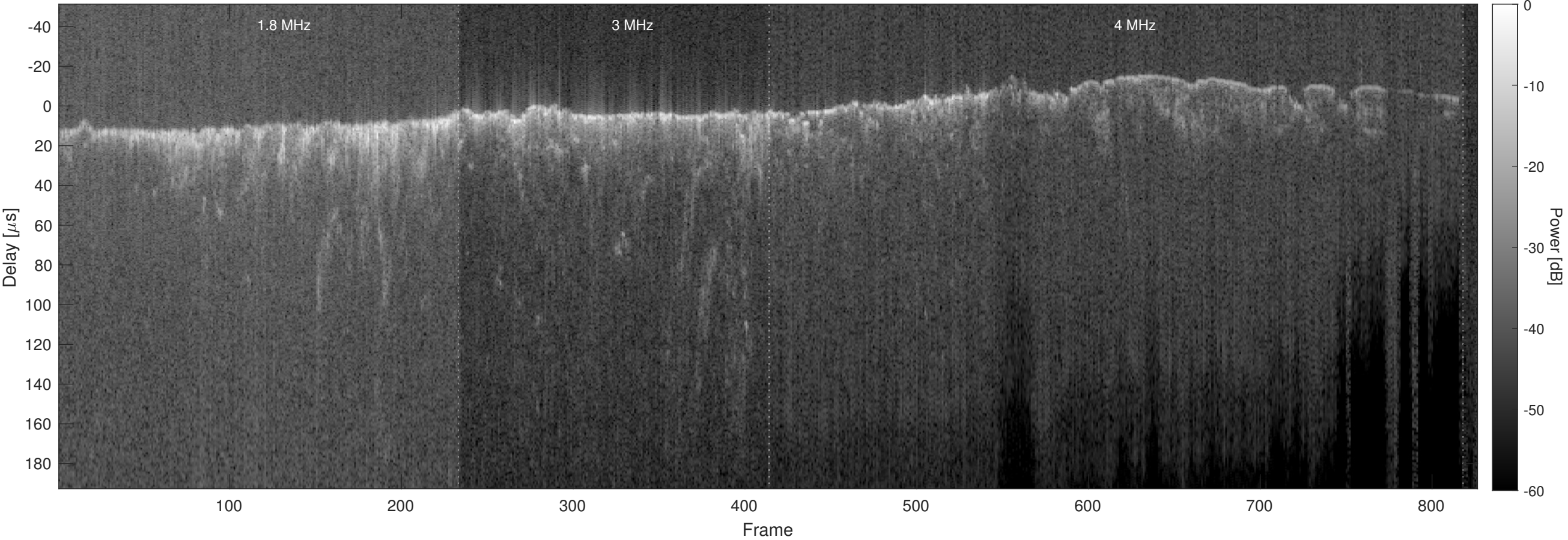
Orbit 6715, Optimized, No Window, Channel 2
