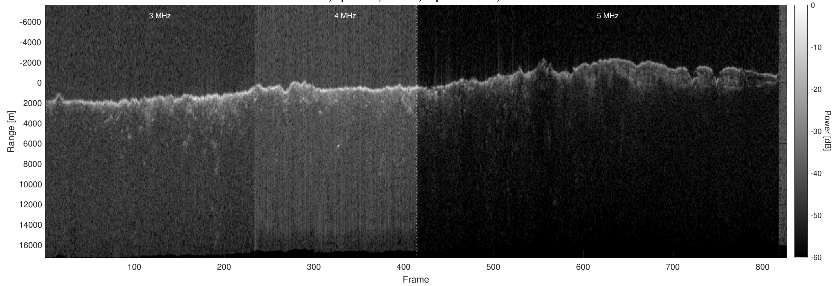
Orbit 6715, Optimized, Window, Depth-Corrected, Channel 2
