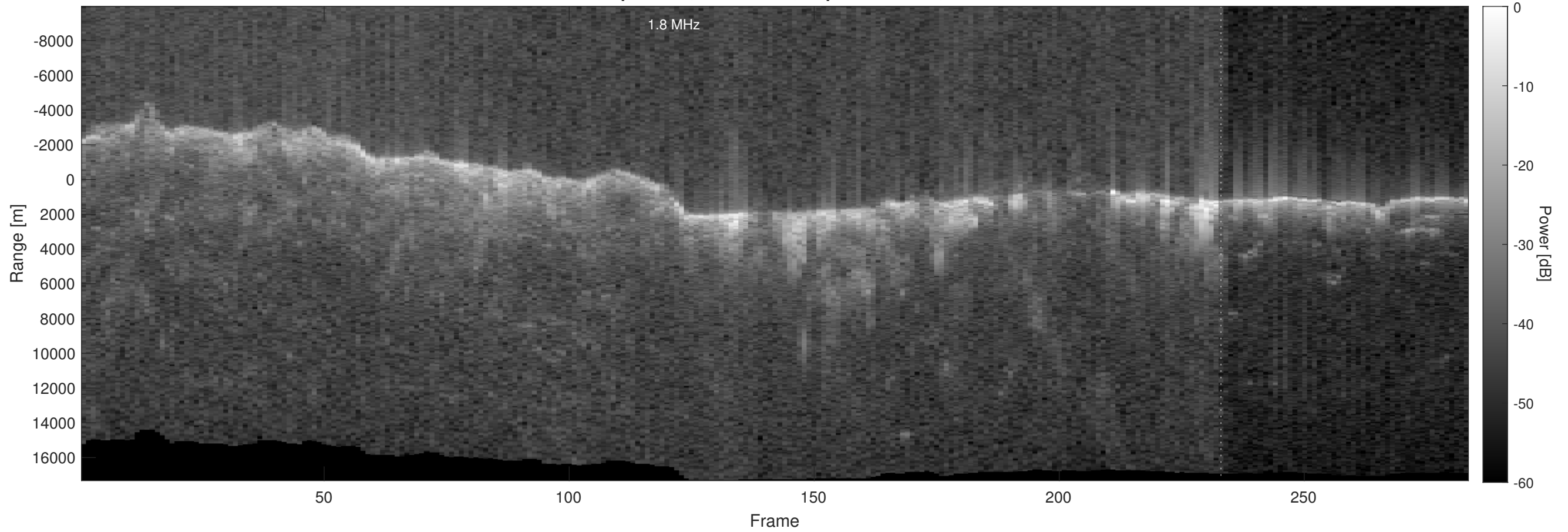
Orbit 6716, Optimized, No Window, Depth-Corrected, Channel 2
