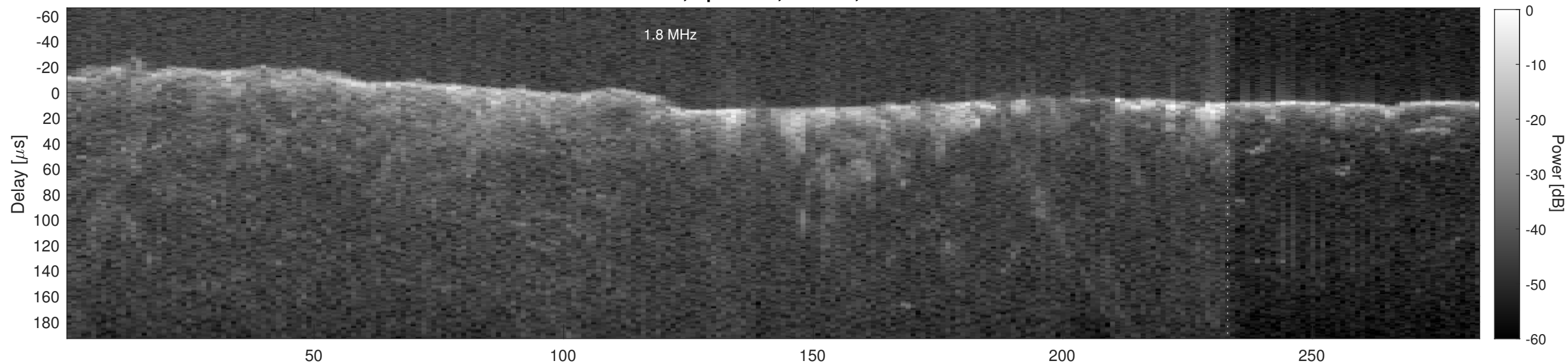
Orbit 6716, Cluttergram
