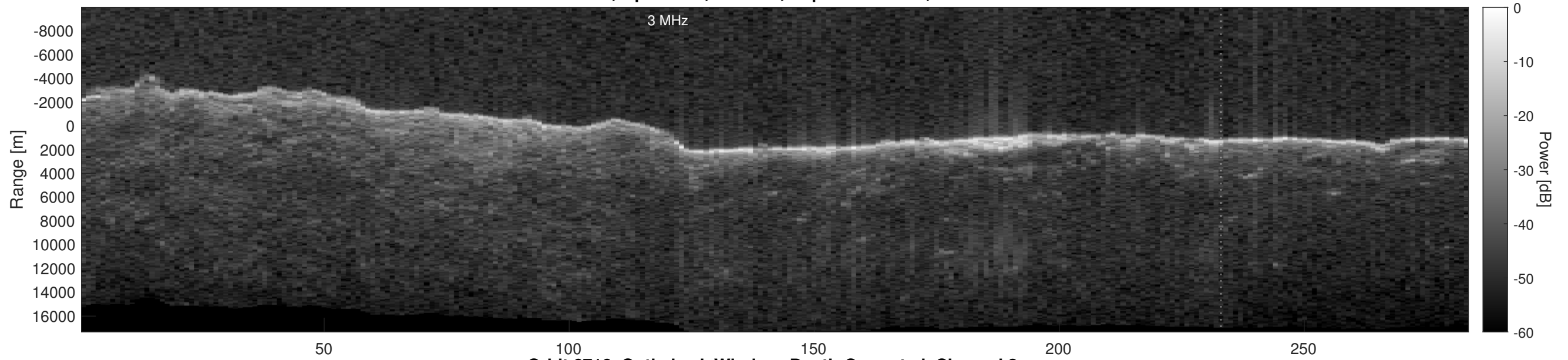
Orbit 6716, Optimized, Window, Depth-Corrected, Channel 2
