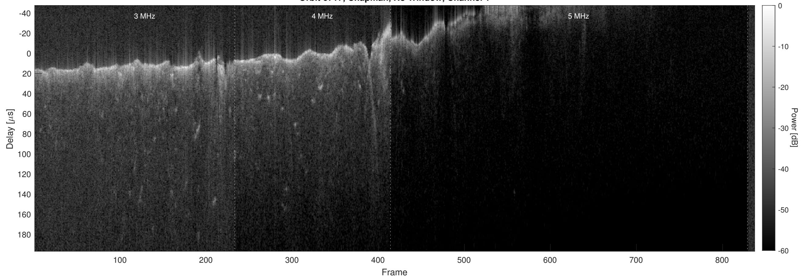
Orbit 6717, Chapman, No Window, Channel 2
