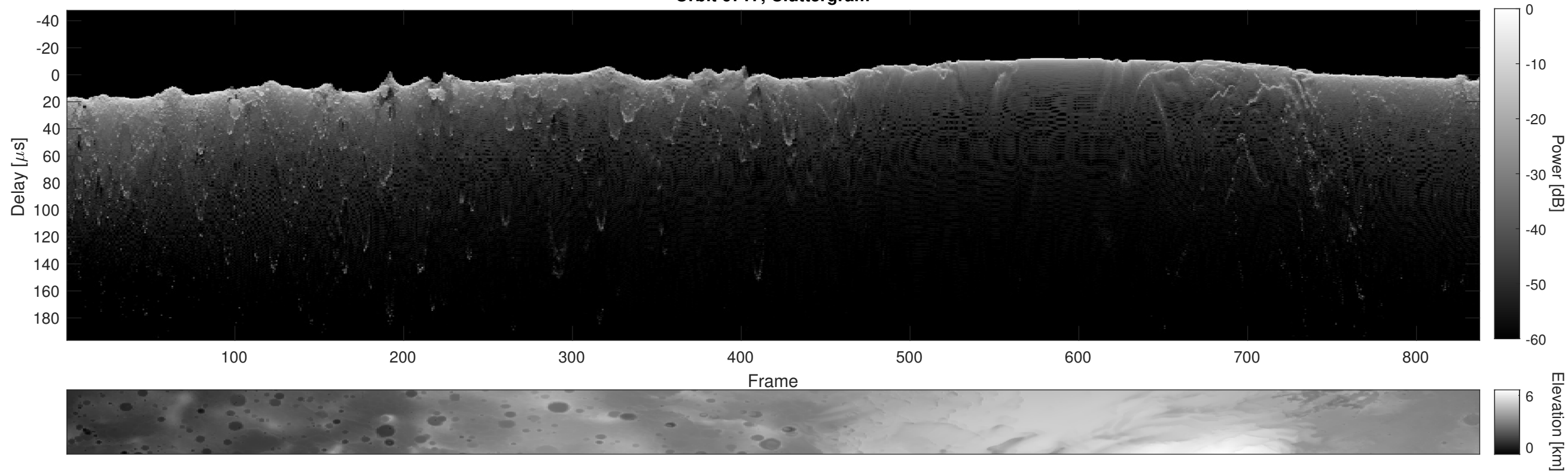
Orbit 6717, Cluttergram
