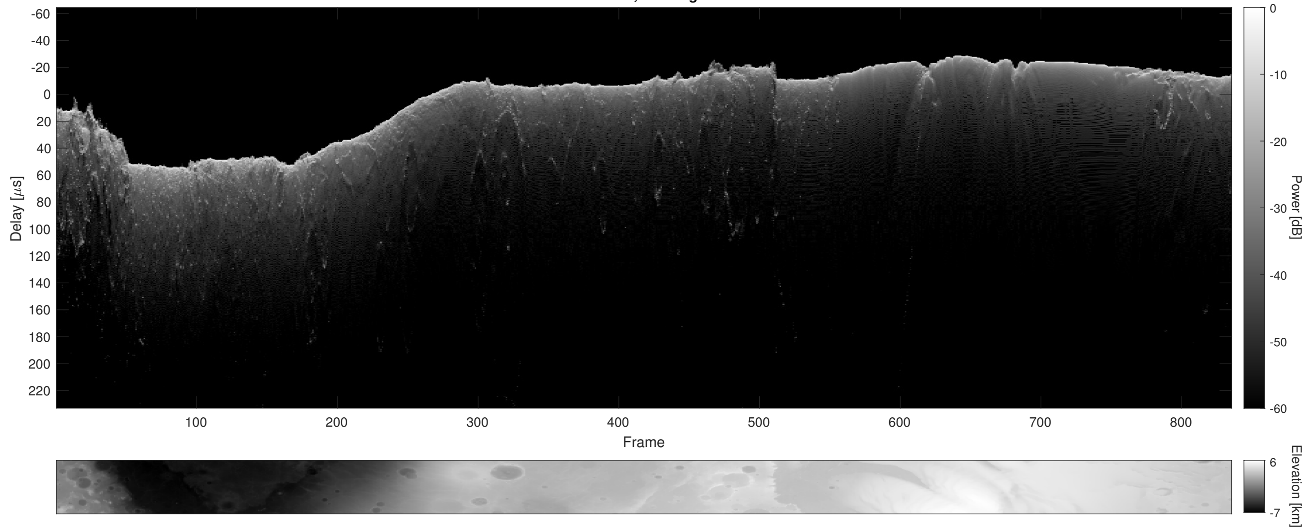
Orbit 6718, Cluttergram
